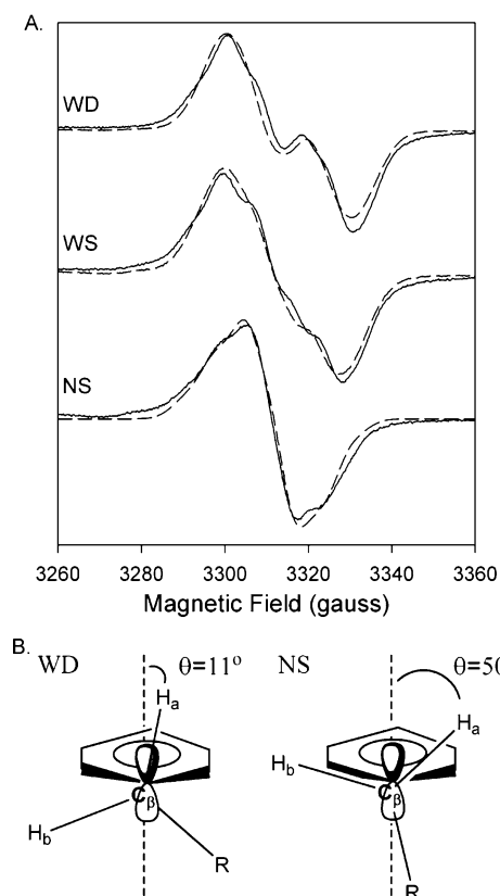
FIGURE 3: (A) Experimental (—) and simulated (---) EPR spectra of the doublet, wide singlet (WS), and narrow singlet (NS) EPR signals from Y348F/Y504F PGHS-2 reacted with peroxide. The doublet was observed after reaction of the double mutant (38 \mu M heme) with 15 equiv of EtOOH for 104 ms. The simulated spectrum represents the sum of 80% of the Y504F WD simulated spectrum and 20% of the NS simulated spectrum. The WS was observed after reaction of the double mutant (15 \mu M heme) with 15 equiv of EtOOH on ice for \sim 10 s. The wide singlet simulation represents the sum of 48% simulated Y504F WD and 52% simulated NS. The NS spectrum was recorded after preincubation of the double mutant (15 \mu M heme) with 5 equiv of nimesulide and subsequent reaction with 15 equiv of EtOOH for 10 s on ice. Parameters for simulation of the Y504F WD and NS spectra are given in Table 3. (B) Structural diagrams of the proposed conformations of the \beta -methylene groups of tyrosyl radicals that give rise to the WD and NS spectra.
