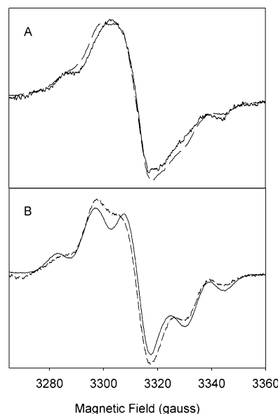
FIGURE 4: EPR spectra of radicals formed during anaerobic reaction of Y348F/Y504F PGHS-2 with AA or d_8 -AA. (A) Reaction at 0 ^\circ C of Y348F/Y504F PGHS-2 (15 \mu M heme) with 15 equiv of EtOOH for 26 s and then with 4 equiv of AA for 11 s (—). The simulated EPR spectrum (---) is an arithmetic combination of 59% Y348F/Y504F PGHS-2 NS and 41% AA-pentadienyl radical. (B) Reaction at 0 ^\circ C of Y348F/Y504F PGHS-2 (15 \mu M heme) with 15 equiv of EtOOH for 19 s and then with 4 equiv of d_8 -AA for 13 s (—). The simulated EPR spectrum (---) is an arithmetic combination of 54% Y348F/Y504F PGHS-2 NS and 46% d_8 -AA-pentadienyl radical. Simulation parameters are given in Table 3 and ref 38.
