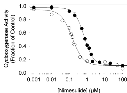
FIGURE 6: Cyclooxygenase inhibition by nimesulide in PGHS-2 (●) and the Y348F/Y504F double mutant (○). The enzyme was preincubated for 1 min at 30^\circ\text{C} with the indicated level of nimesulide before the reaction was initiated by addition of arachidonate ( 100 \mu\text{M} ). Activities are normalized to uninhibited control values; data represent averages of triplicate measurements, and standard deviations are indicated by error bars.
