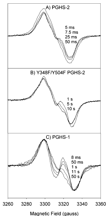
FIGURE 8: EPR spectra of tyrosyl radicals formed during reaction of PGHS-2, Y348F/Y504F PGHS-2, and PGHS-1 with EtOOH. Individual EPR spectra are scaled to the same amplitude and overlaid to facilitate line shape comparisons. (A) PGHS-2 (11.2 \mu M heme) in 100 mM KP_i (pH 7.2), 0.1% Tween-20, and 10% glycerol was reacted at room temperature with 5 equiv of EtOOH for the indicated times. Data are from ref 27. (B) The Y348F/Y504F PGHS-2 double mutant (68 \mu M heme) in 100 mM KP_i (pH 7.2), 50 \mu M phenol, 0.04% octyl glucoside, and 10% glycerol was reacted at room temperature with 15 equiv of EtOOH for the indicated times. (C) PGHS-1 (8.5 \mu M heme) in 100 mM KP_i (pH 7.2), 0.1% Tween-20, and 10% glycerol was reacted at room temperature with 5 equiv of EtOOH for the indicated times. Data are from ref 27.
