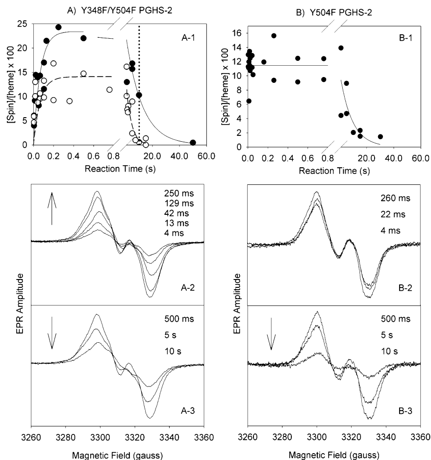
FIGURE 2: Tyrosyl radical kinetics during the reaction of Y348F/Y504F PGHS-2 and Y504F PGHS-2 with EtOOH. (A) The double mutant (68 \mu M heme) in 100 mM \text{KPi} (pH 7.2), 50 \mu M phenol, 0.04% octyl glucoside, and 10% glycerol was reacted at room temperature with 15 equiv of EtOOH. (A-1) Time course of Y348F/Y504F tyrosyl radical intensity as determined by double integration of the EPR signals ( \bullet ) in experiments with two separate enzyme preparations and time course for the PGHS-2 Y148F/Y348F/Y404F/Y504F quadruple mutant ( \circ ) (25). (A-2 and A-3) EPR spectra from the double mutant reaction samples freeze trapped at the indicated times. (B) Y504F PGHS-2 (48 \mu M heme) was reacted with 15 equiv of EtOOH at room temperature (25). (B-1) Time course of radical intensity determined by double integration. (B-2 and B-3) EPR spectra from the Y504F mutant reaction samples freeze trapped at the indicated times.
